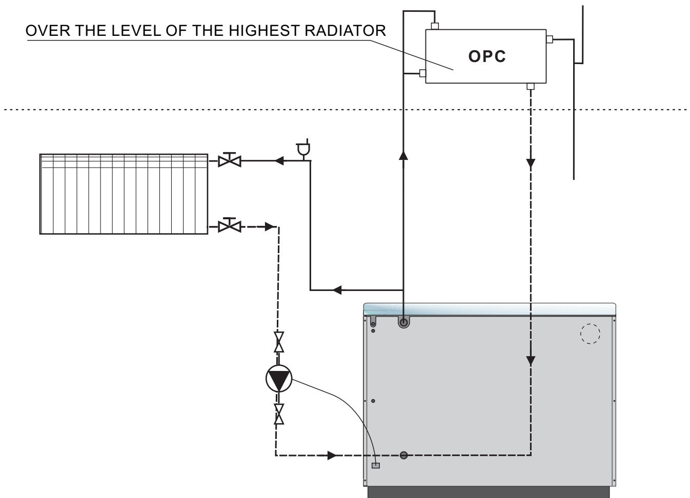
Diagram 1. Connecting an BIO-PEK B - L (applies to BIO-PEK B - D)
